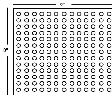
Holes are tapped @ 10-32 on 1/2" spacing
